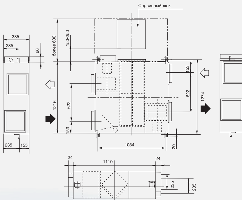
ERV0800AAN, ERV1000AAN
